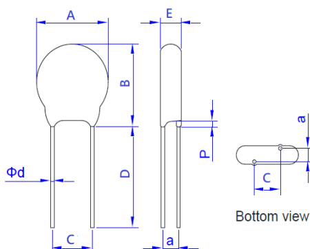
Straight Lead Type (S)
